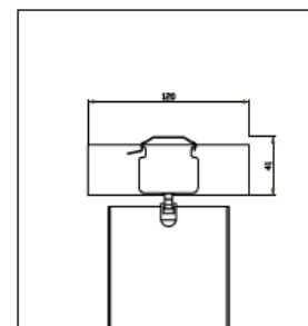
Head rail side view Detalle perfil cabezal
